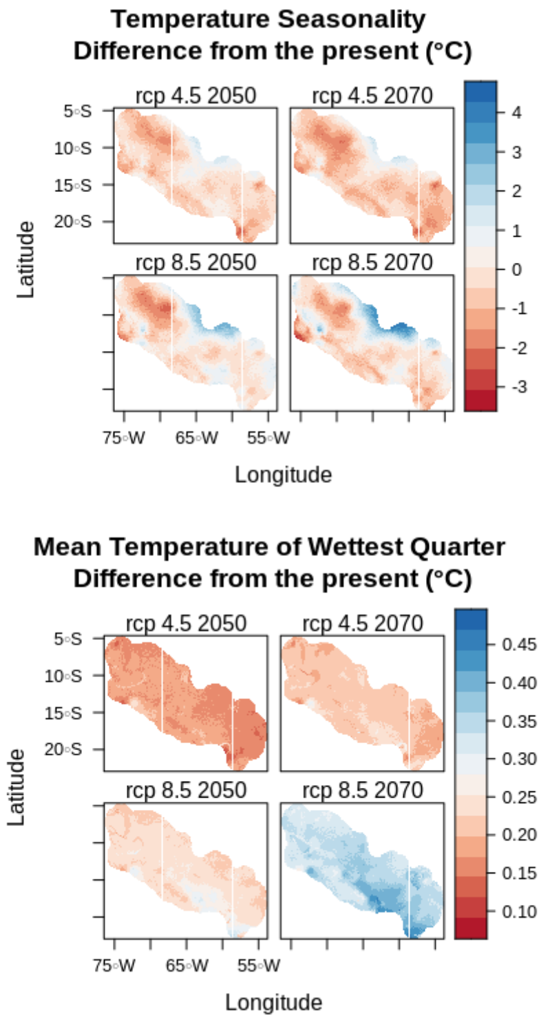
Fig.A8.8: Difference between current and future of the four bioclimatic variables used in niche modeling. These values were extracted from the raster used in this study. (RCP: Representative Concentration Pathway)
